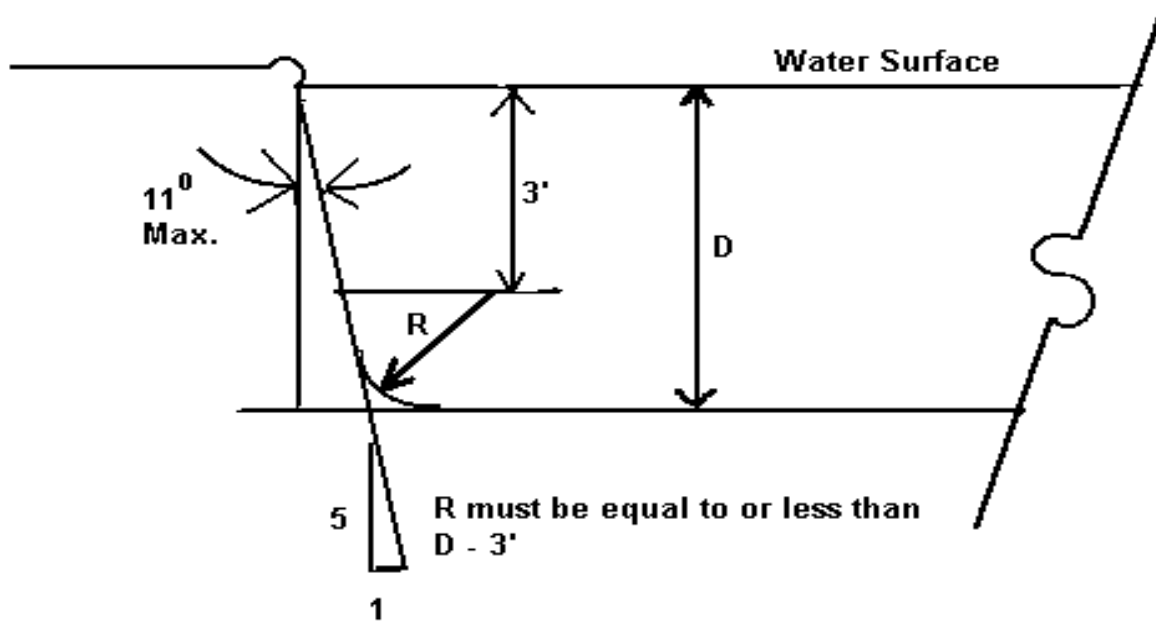
Illustration of Pool Side Wall
